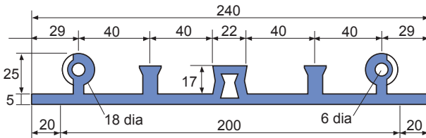
7.5 m long coil, weight 23 kg
