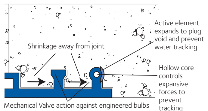
AT System with Active Element
