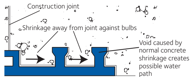
Conventional Waterstop
